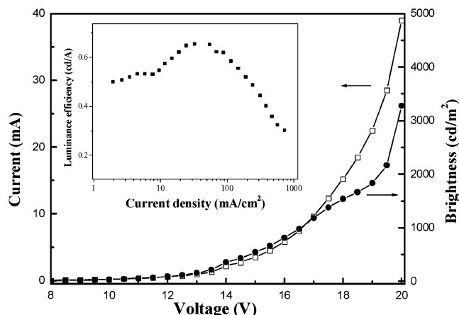
Figure 6. Current–brightness–voltage characteristics of the device (ITO/PEDOT/MeLPF/Ba/Ag). Inset: dependence of the luminance efficiency on the drive current density for the device.
